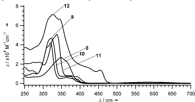
Figure 4. UV/Vis absorption spectra in \text{CH}_2\text{Cl}_2 .
