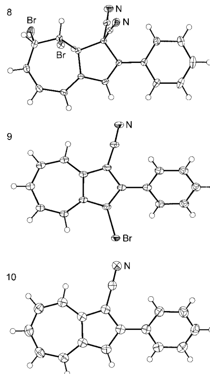
Figure 1. X-ray crystal structures of 8 , 9 , and 10 .
