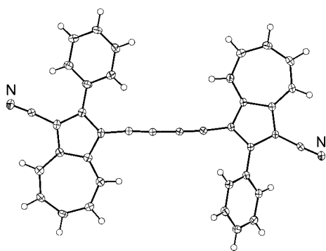
Figure 3. Crystal structure of 12 .
